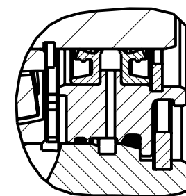
DETAIL A DUAL SHAFT SEAL ASSEMBLY P2-105-0210-02□
