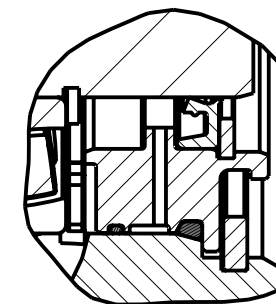
DETAIL A SINGLE SHAFT SEAL ASSEMBLY P2-105-0210-01□
